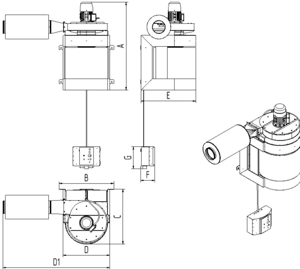
Fig. 17: Dimensions sheet
