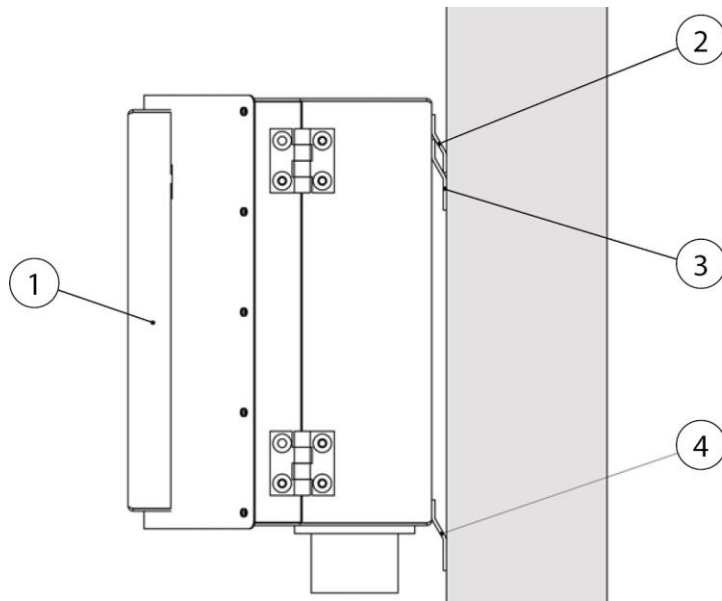
Fig. 8: Mounting the control box
