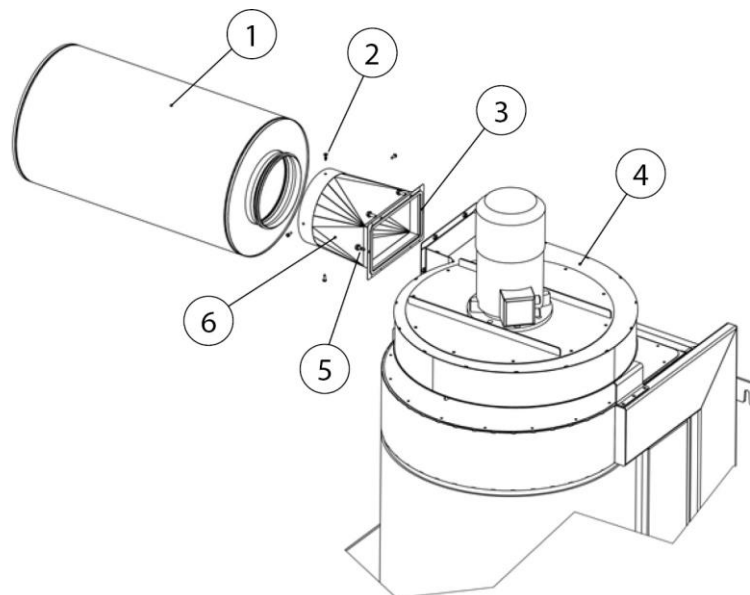
Fig. 6: Mounting the silencer
